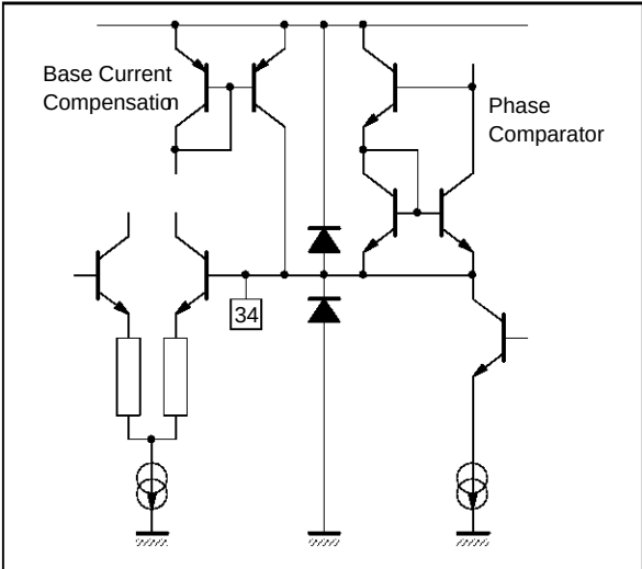
Figure 19 : Pin 34 (CLPF)
