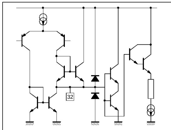
Figure 14 : Pin 32 (CKP)
