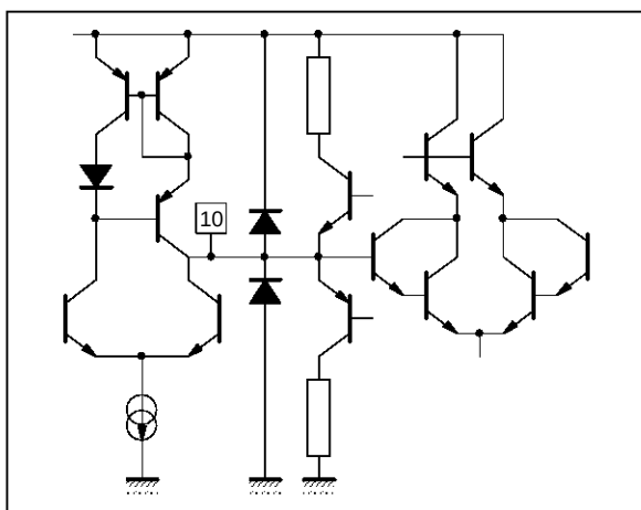
Figure 5 : Pin 10 (SLPF)
