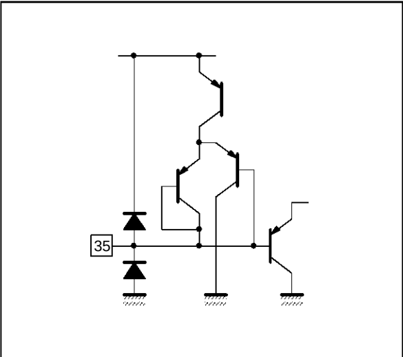
Figure 20 : Pin 35 (FBL)
