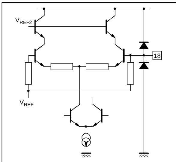
Figure 13 : Pin 18 (PALIN)
