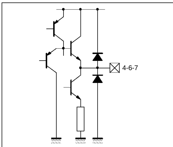
Figure 5 : Pin 10 (SLPF)
