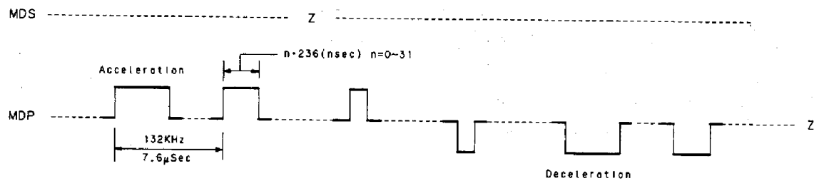
Timing Chart 1-6
