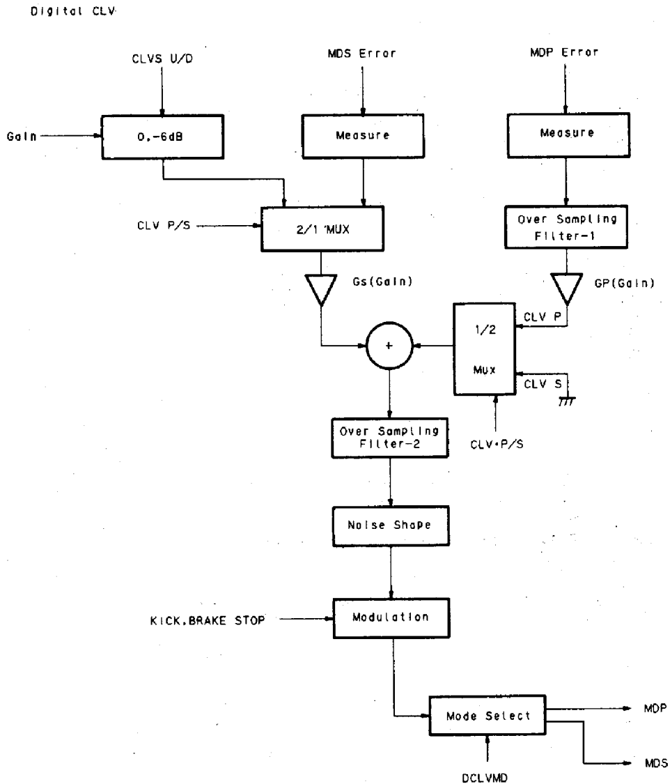
Figure 3-14 Block diagram
