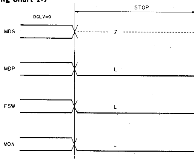
Timing Chart 1-7
