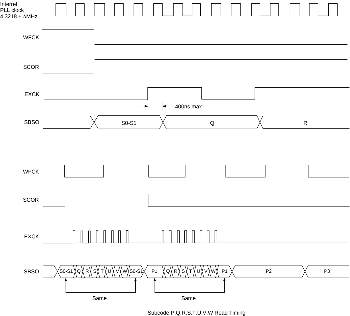
Timing Chart 2-1
