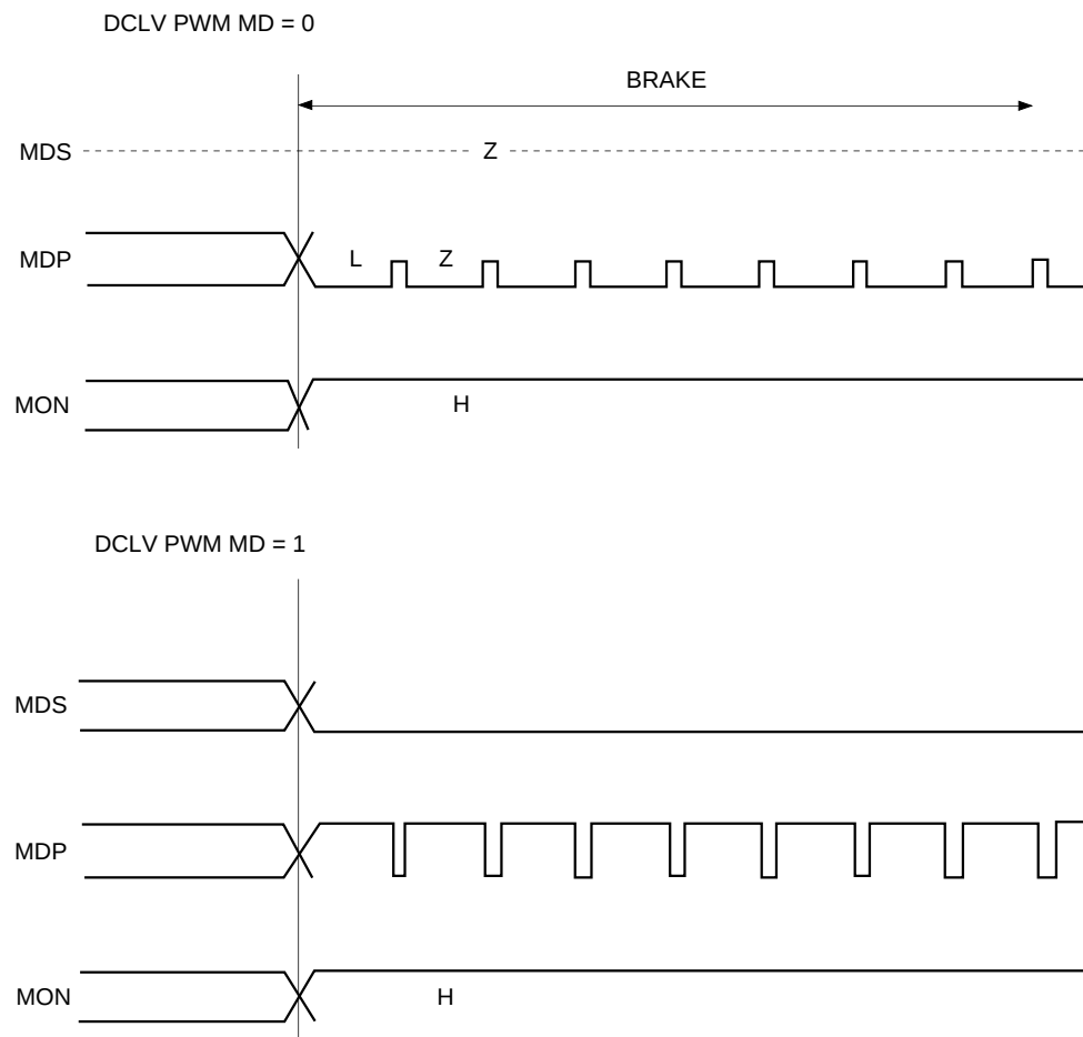
Timing Chart 1-8
