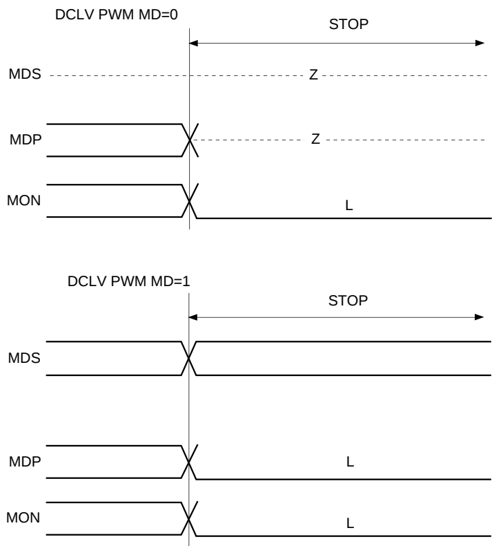
Timing Chart 1-6
