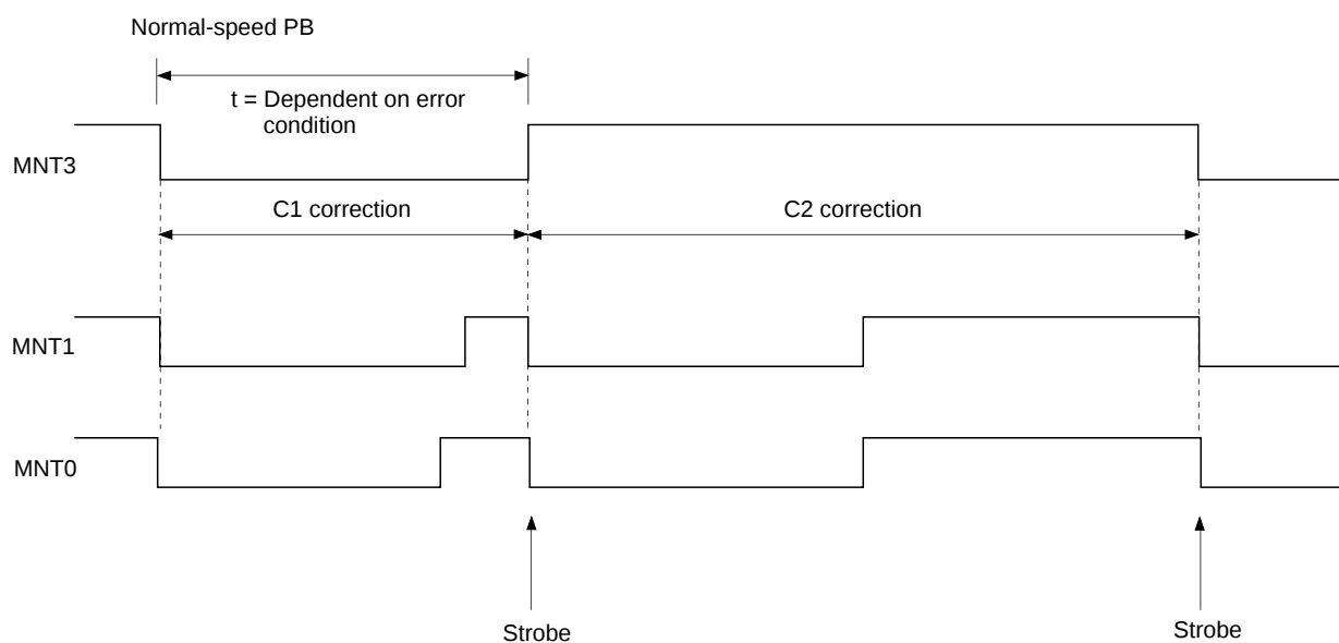
Timing Chart 4-1
