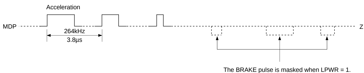
Timing Chart 1-10
