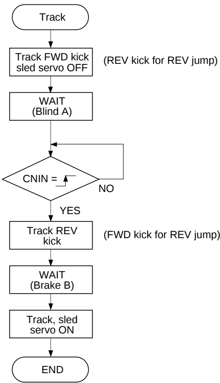
Fig. 4-4-(a). 1-Track Jump Flow Chart
