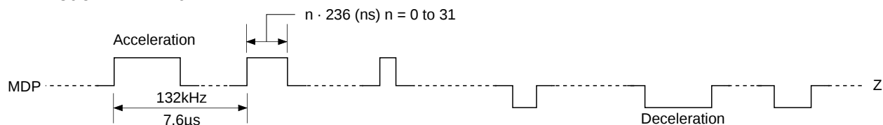
Timing Chart 1-7
