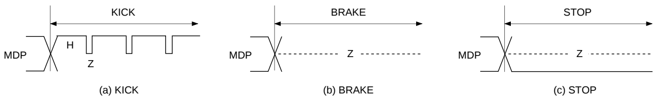
Timing Chart 1-4 CLV-W mode (when following the spindle rotational velocity) LPWR = 1
