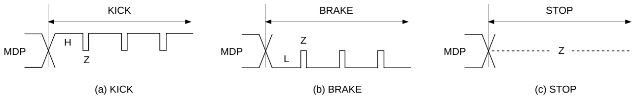
Timing Chart 1-2 CLV-N mode LPWR = 0
