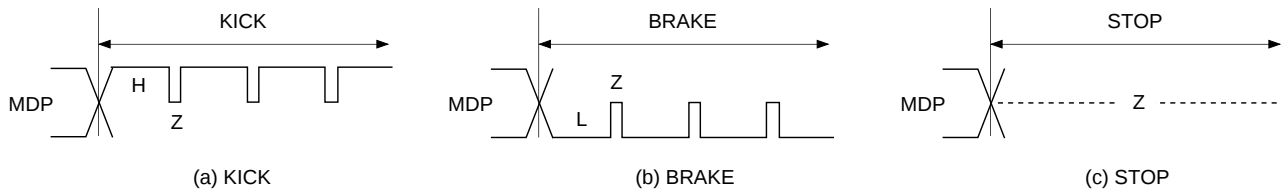
Timing Chart 1-3 CLV-W mode (when following the spindle rotational velocity) LPWR = 0
