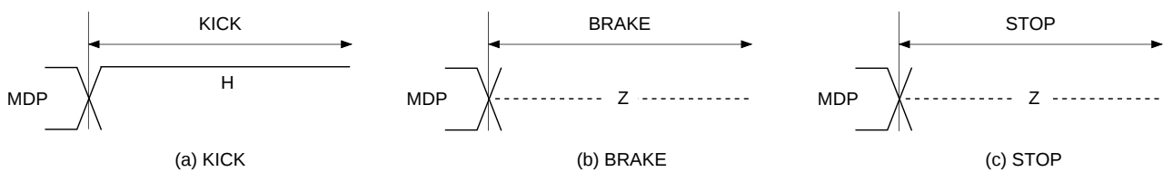
Timing Chart 1-6 CAV-W mode LPWR = 1
