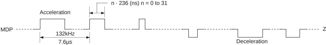
Timing Chart 1-7
