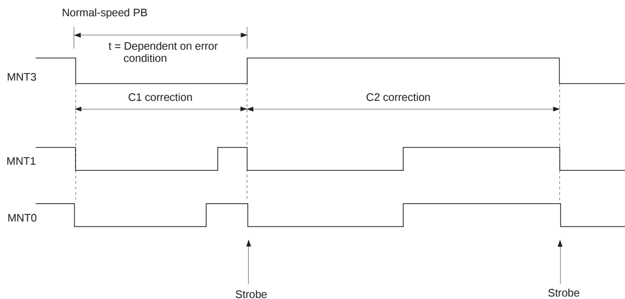
Timing Chart 4-1
