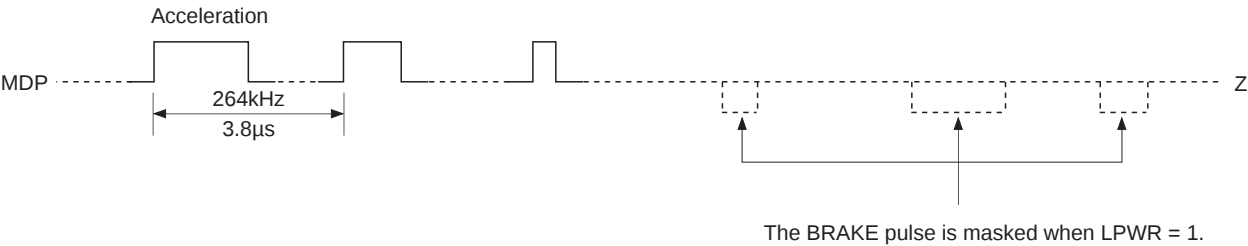
Timing Chart 1-10
