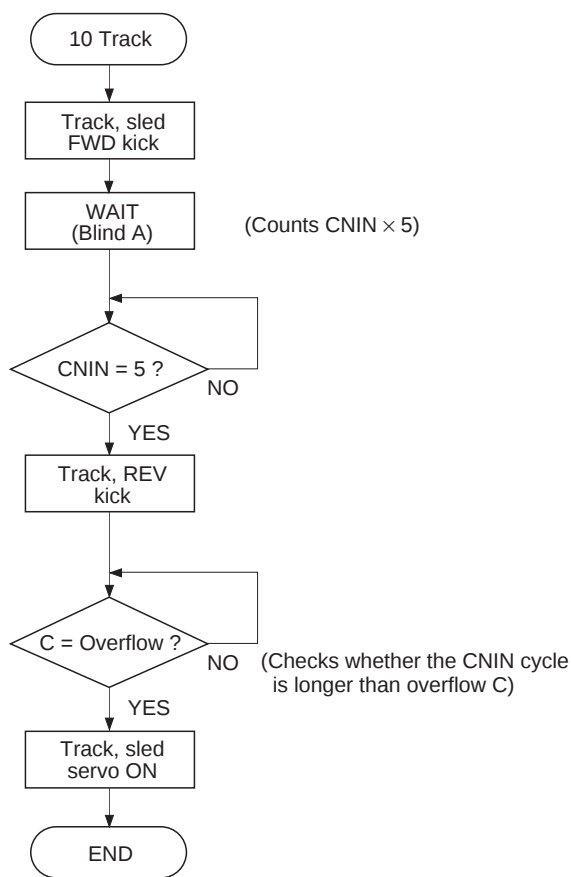
Fig. 4-5-(a). 10-Track Jump Flow Chart
