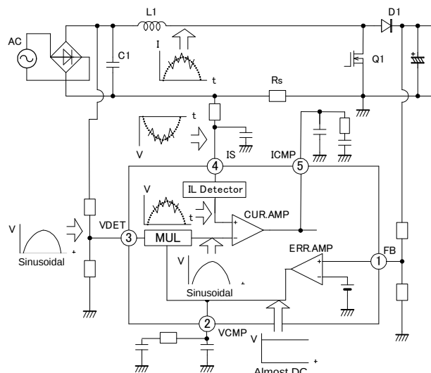
Fig.3 Aspects of waveforms at different parts
