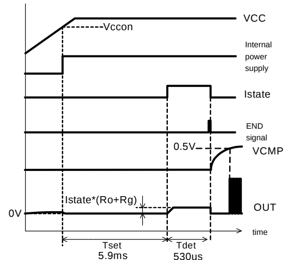
Fig.6 Frequency setting sequence
