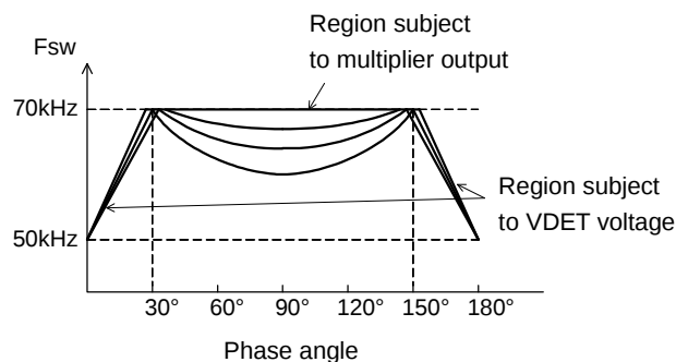
Fig.8 Oscillation frequency vs. phase angle
