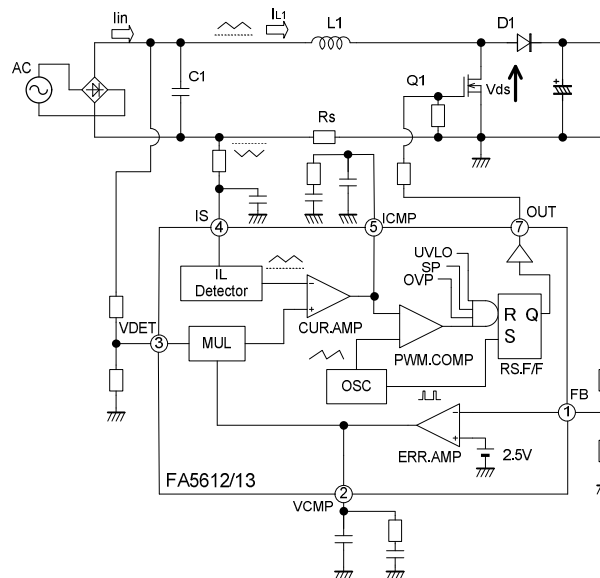
Fig.1 Block diagram of operating circuit
