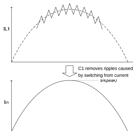
Fig.4 Power factor corrected waveform
