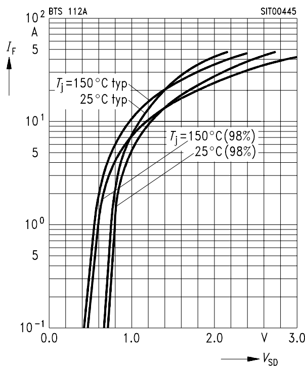
Forward characteristics of reverse diode I_F = f(V_{SD}) Parameter: T_j, t_p = 80\text{ }\mu\text{s}
